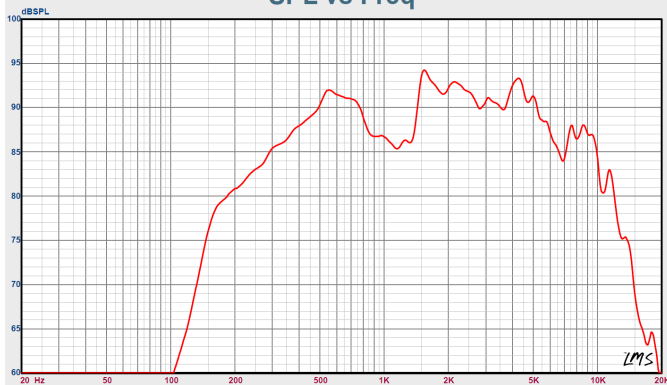
Sound pressure levels at 1W/1m P-5/15 PS SPL vs Freq
