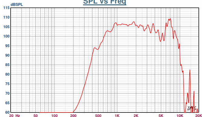
Sound pressure levels at 1W/1m (MP-28-54)
