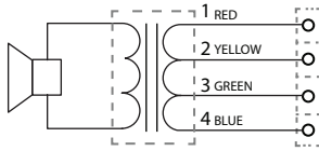
Fig. 2 - Circuit Diagram
