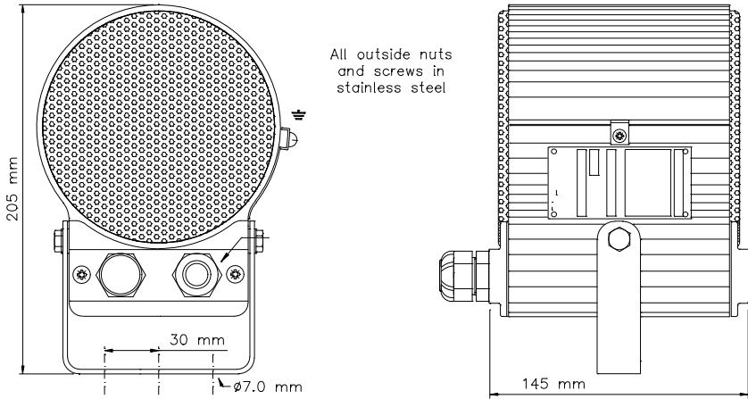
Fig. 1 - Technical drawing
