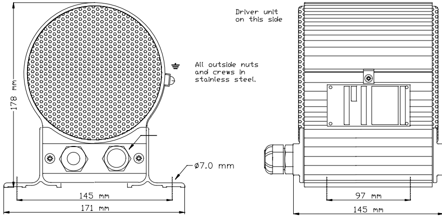
Fig. 1 - Technical drawing
