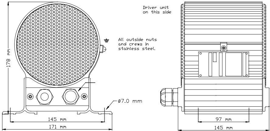
Fig. 1 - Technical drawing
