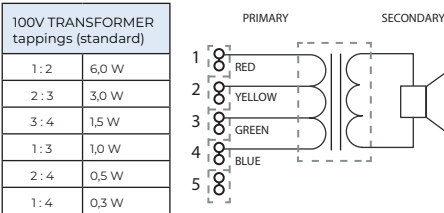
Fig. 2 - Circuit Diagram
