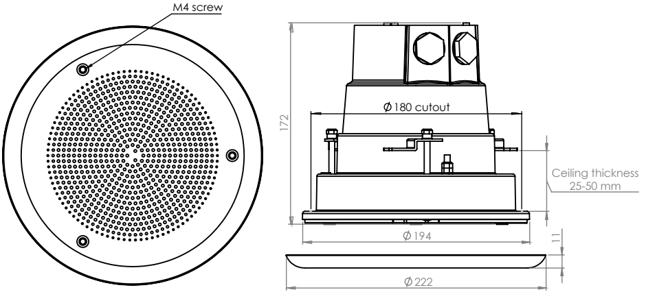
Fig. 1 - Technical drawing
