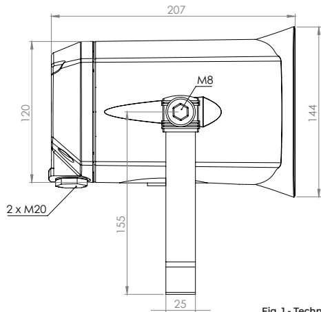
Fig. 1 - Technical drawing
