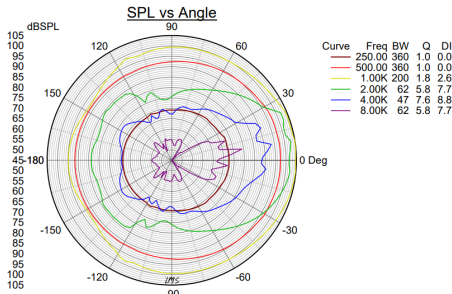
Fig. 4 - Polar plot 1W/1m
