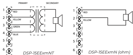
Fig. 2 - Circuit Diagram
